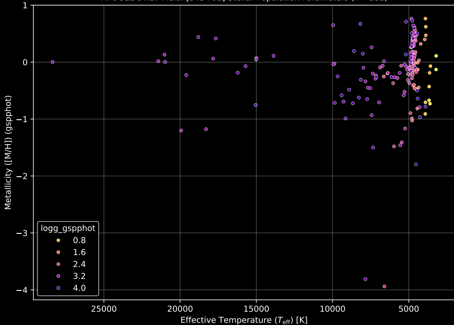
APOGEE DR17 Field: [345+02] Stellar Population Parameters (n= 182)
