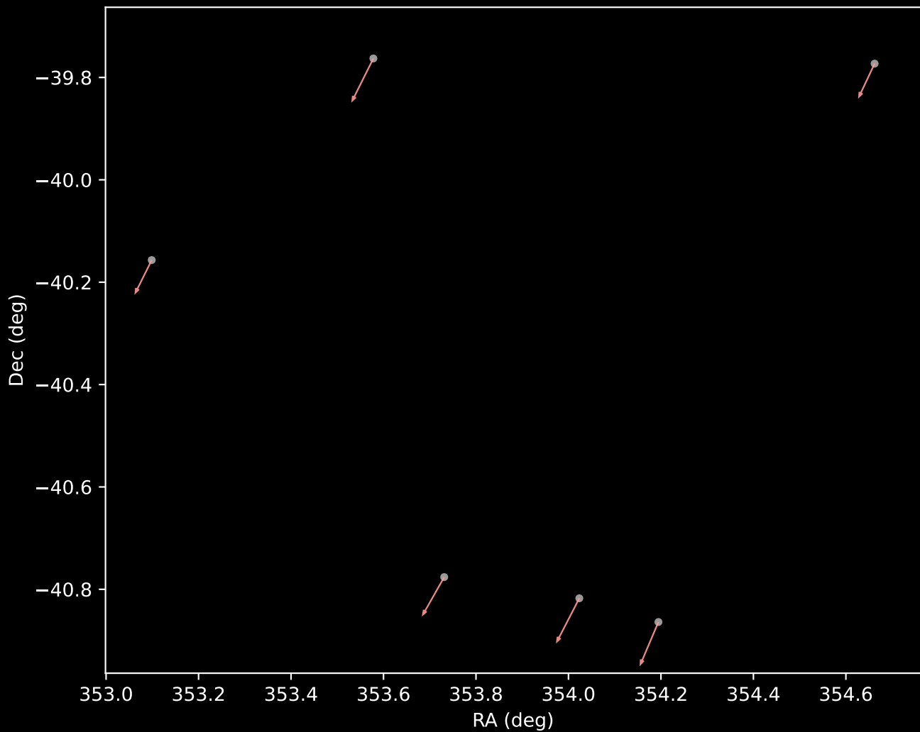
APOGEE DR17 Cluster 7 Proper Motion Vectors (n=6)
