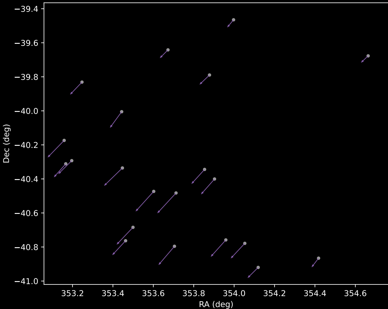
APOGEE DR17 Cluster 8 Proper Motion Vectors (n=21)
