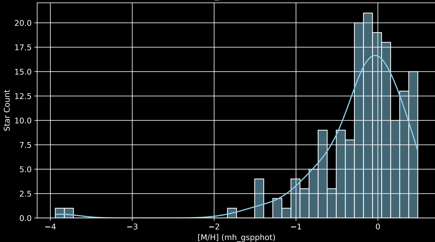
APOGEE DR17 Field: [345+02 [M/H] (mh_gspphot) (n= 167)
