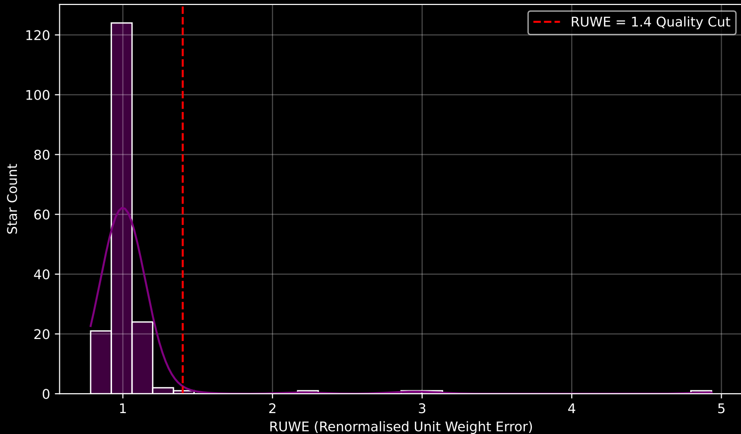
GAPOGEE DR17 Field [345+02] RUWE Distribution (n= 176)
