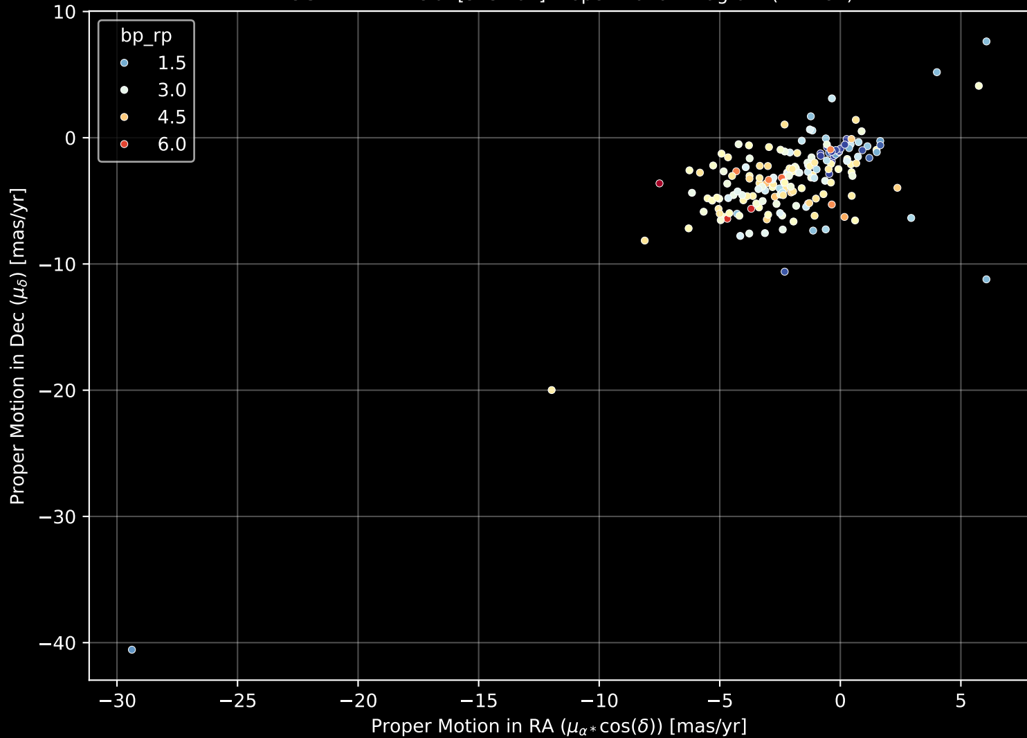
APOGEE DR17 Field: [345+02] Proper Motion Diagram (n= 182)
